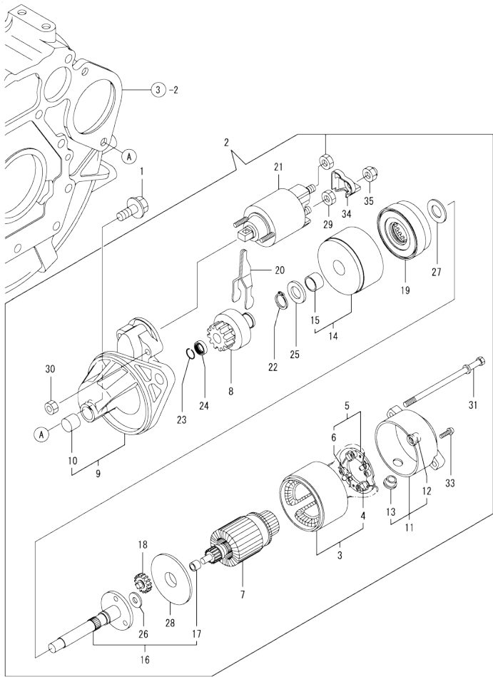
Fig.14. STARTING MOTOR
