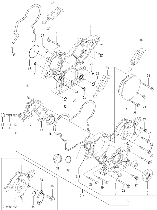
Fig.2. GEAR HOUSING
