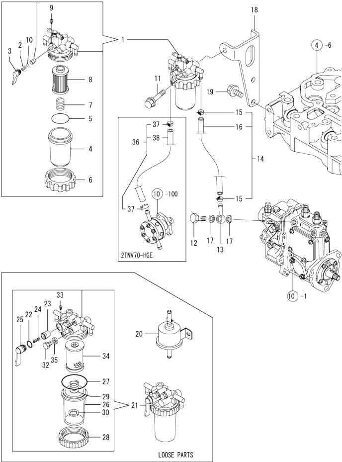
Fig.13. FUEL LINE
