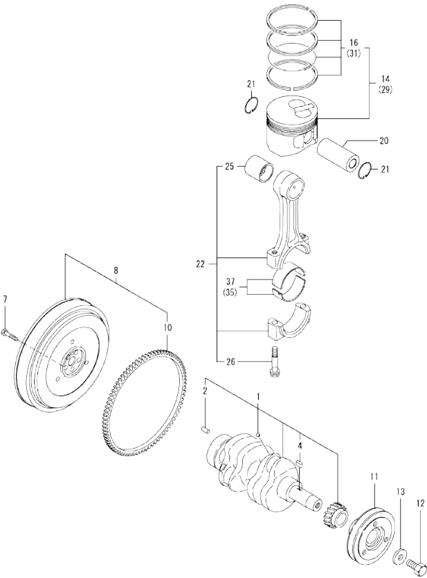
Fig.7. CRANKSHAFT & PISTON
