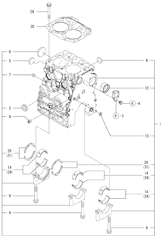
Fig.1. CYLINDER BLOCK
